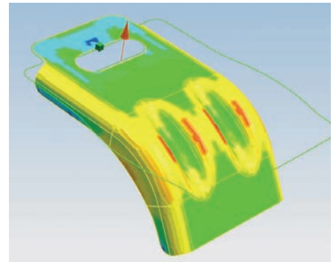
Stress results.
