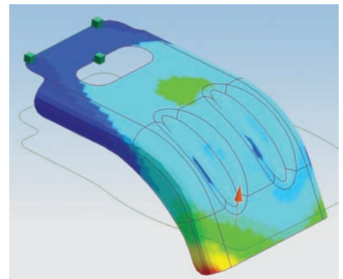
Springback results.
