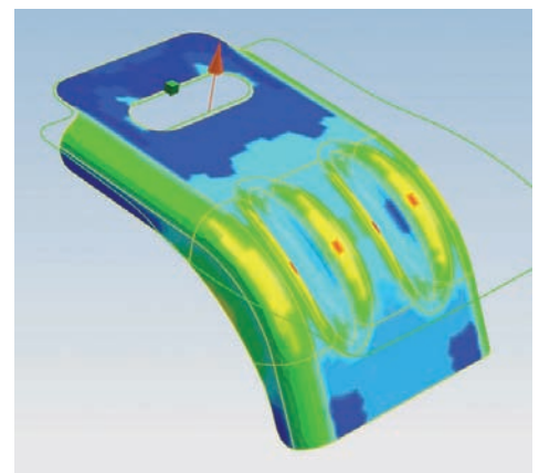
Strain results.
