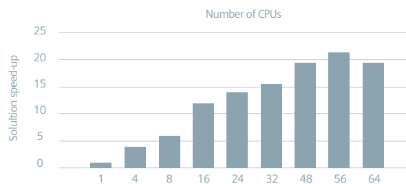
Trimmed car body – 2.3 million degrees of freedom, 380,000 node points, 900 mode shapes IBM P650 workstation cluster 64 POWER4 (1.5 GHz) CP
